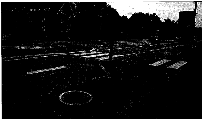
FIGURE 12-6. A choker is a narrowing of the street, either at an intersection or midblock, in order to reduce the width of the traveled way.
