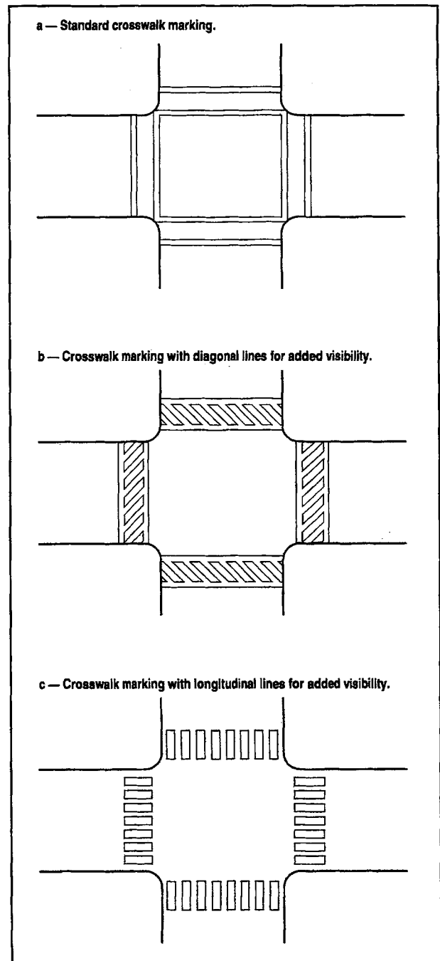
FIGURE 6-1. Typical crosswalk markings. 1
