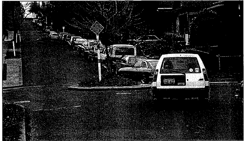
FIGURE 12-4. Traffic circles (minicircles) separate points of conflict within an intersection and often slow speeds of vehicular traffic.
