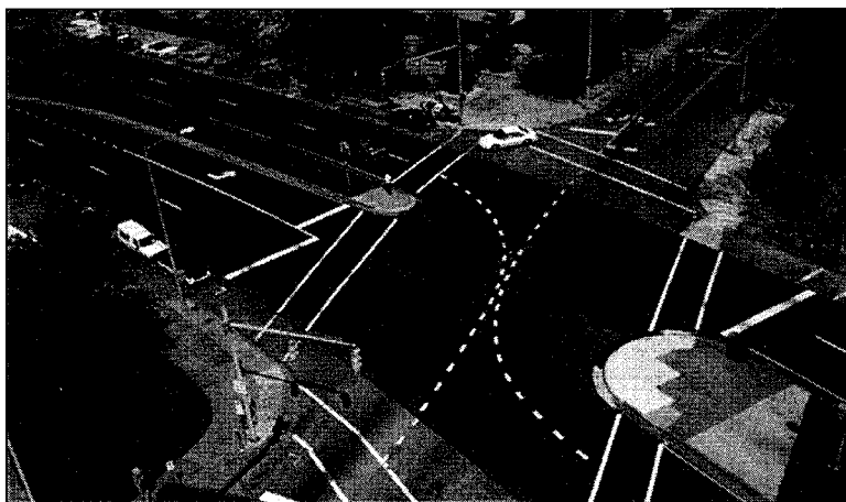
FIGURE 7-3. Pedestrian refuge islands can create a safer crossing for wide streets.
