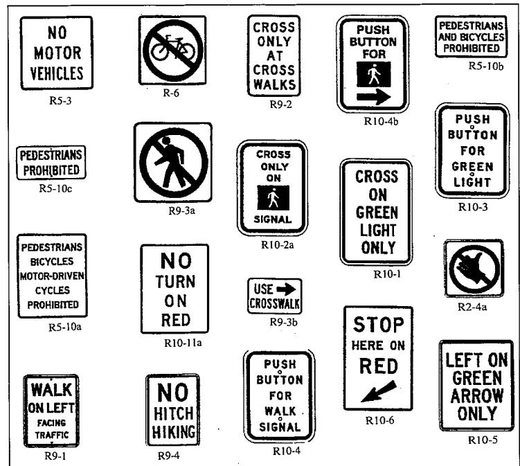
FIGURE 4-1. Typical regulatory signs relating to pedestrians. 1
