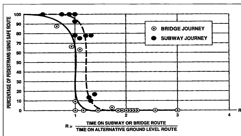
FIGURE 10-4. Pedestrian use of grade separated crossing.
