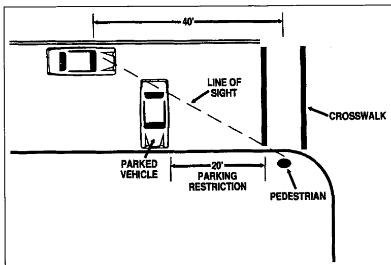
FIGURE 9-6. Pedestrian sight distance and parking restrictions.
