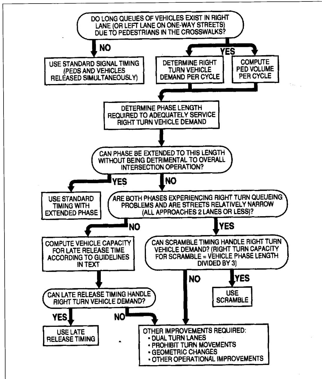
FIGURE 5-7. Flow chart for selecting pedestrian signal phasing. Reprinted with permission. Source: C. M. Abrams and S. A. Smith. Selection of Pedestrian Signal Phasing . In Transportation Research Record 629, Transportation Research Board, National Research Council, Washington, D.C., 1977.
