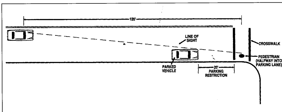
FIGURE 9-5. Pedestrian sight distance and parking restrictions.
