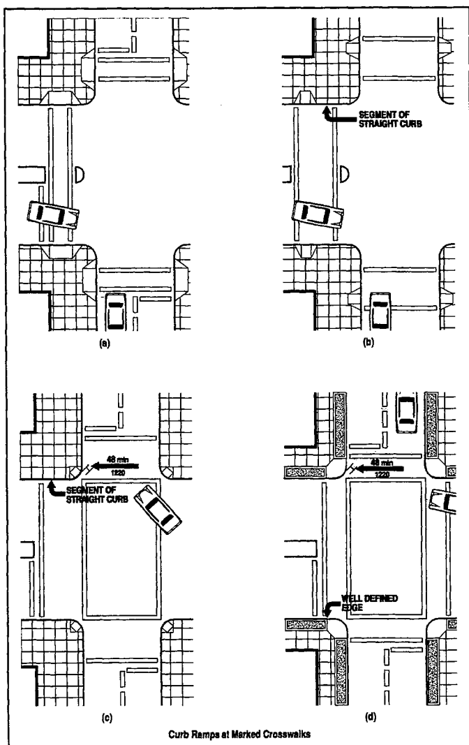
FIGURE 6-7. Guidelines for crossing placement at intersections. 6
