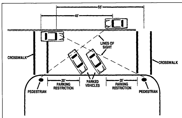
FIGURE 9-7. Pedestrian sight distance and parking restrictions needed for 60 degree angle parking.
