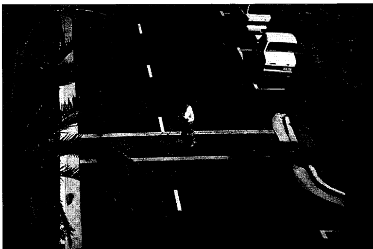
FIGURE 1-7. Extended or flared curbs can shorten the crossing distance for pedestrians and provide improved visibility between motorists and pedestrians.
