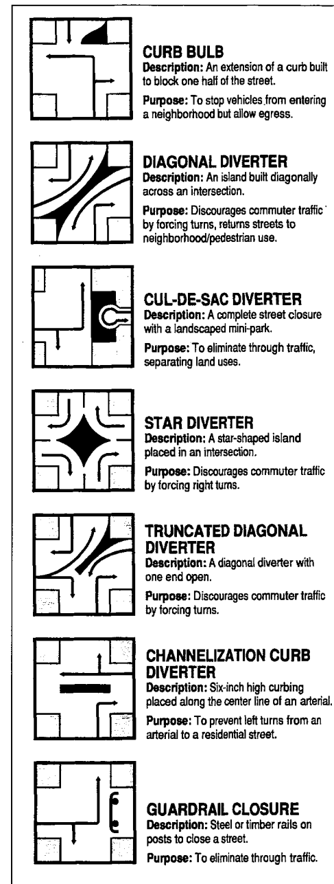
FIGURE 12-1. Neighborhood traffic control measures: Types of diverters.
