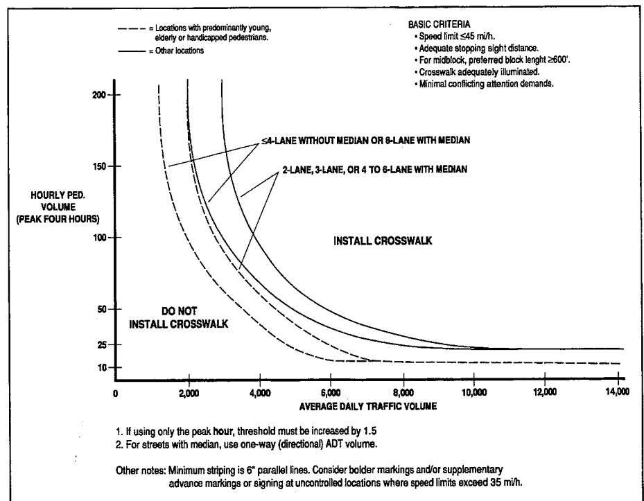
FIGURE 6-2. Guidelines for the installation of marked crosswalks at uncontrolled crossings. Reprinted with permission. Source: Steven A. Smith and Richard L. Knoblauch. Guidelines for the Installation of Crosswalk Markings. In Transportation Research Record 1141, Transportation Research Board, National Research Council, Washington, D.C., 1987.
