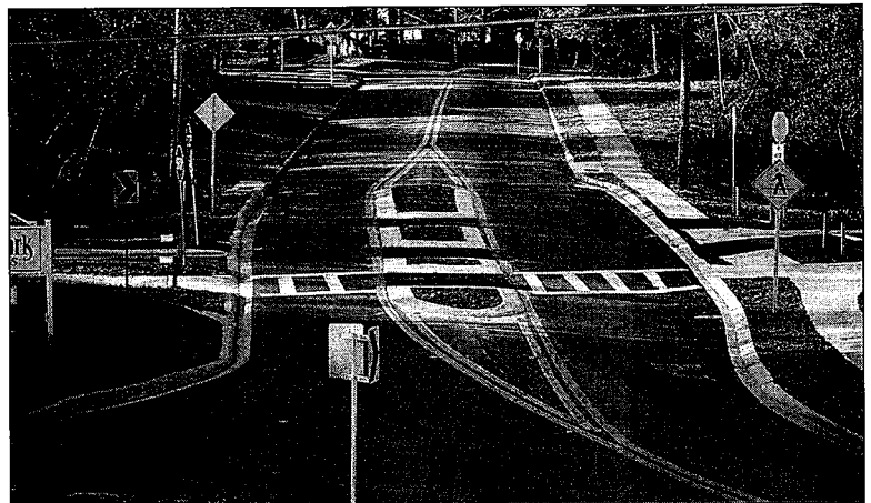
FIGURE 7-5. Cut-through ramps should be provided on refuge islands and medians to accommodate wheelchair users.
